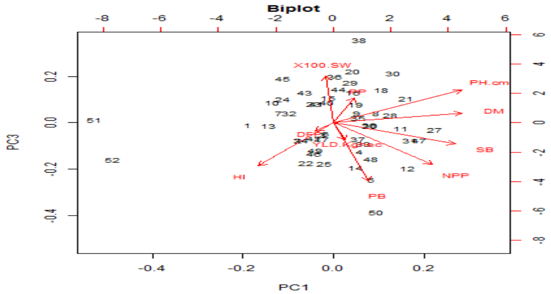
Figure 3. Biplot of PC1 and PC3 showing contribution of various traits in variability.
