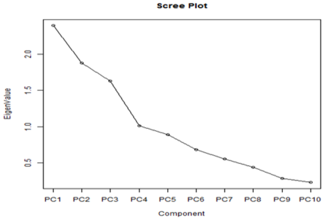
Figure 1. Scree plot showing contributions of PCs in variability.
