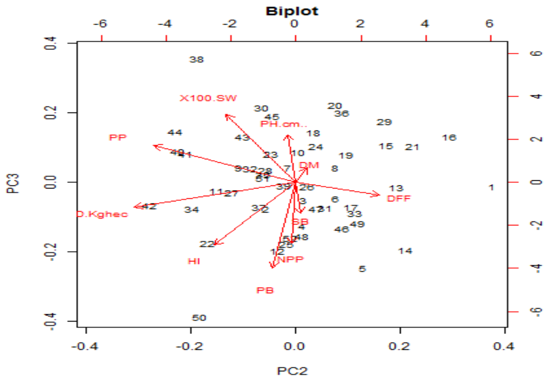
Figure 4. Biplot of PC2 and PC3 showing contribution of various traits in variability.
