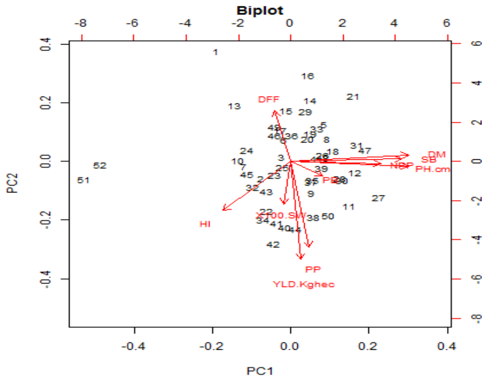
Figure 2. Biplot of PC1 and PC2 showing contribution of various traits in variability.
