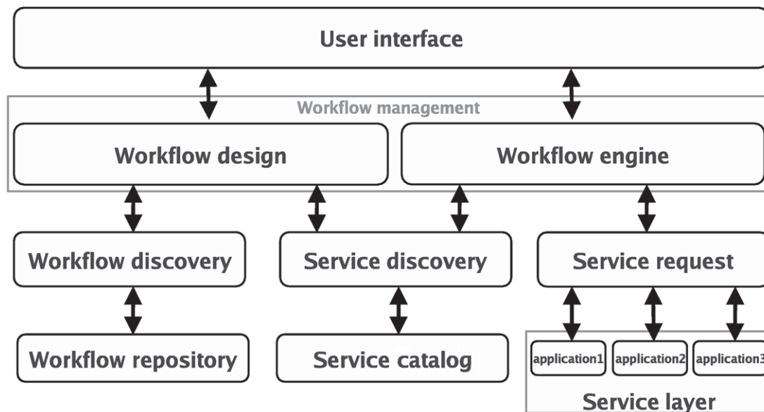
Figure 2. Framework architecture.
